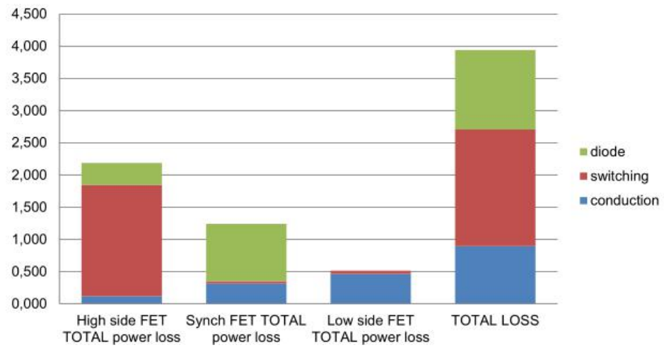
OVERALL SWITCHING LOSS DISTRIBUTION
